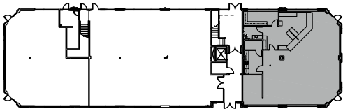
BUILDING PLAN
